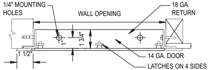
SECTION DETAIL
